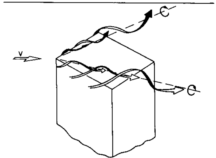
Figure 2 Roof vortex formation for wind at 45 degrees to building walls
