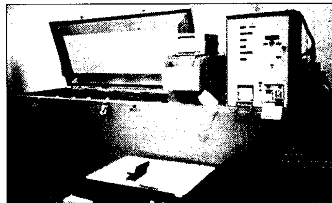
Figure 4. Freeze-thaw apparatus.
