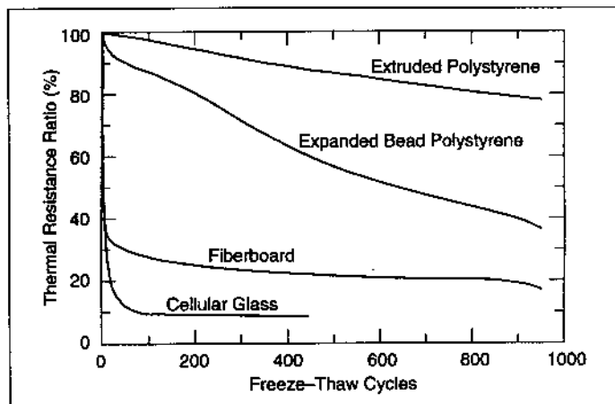
Figure 9. Thermal resistance ratio (TRR)-freeze-thaw cycle relationships for the four insulations shown in Figure 8.
